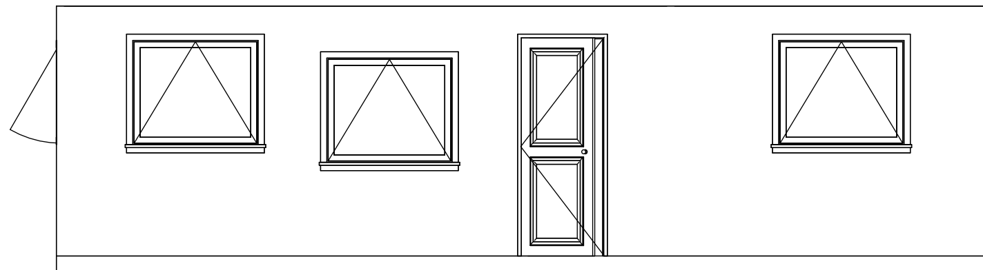
3 South 1 : 50
